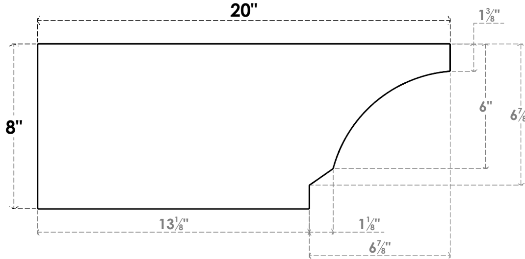
SIDE PROFILE
